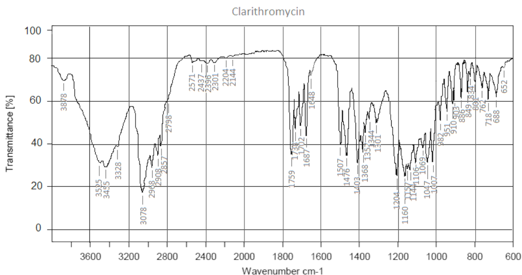
Figure 13.2: FTIR Spectra of Clarithromycin CLAR
