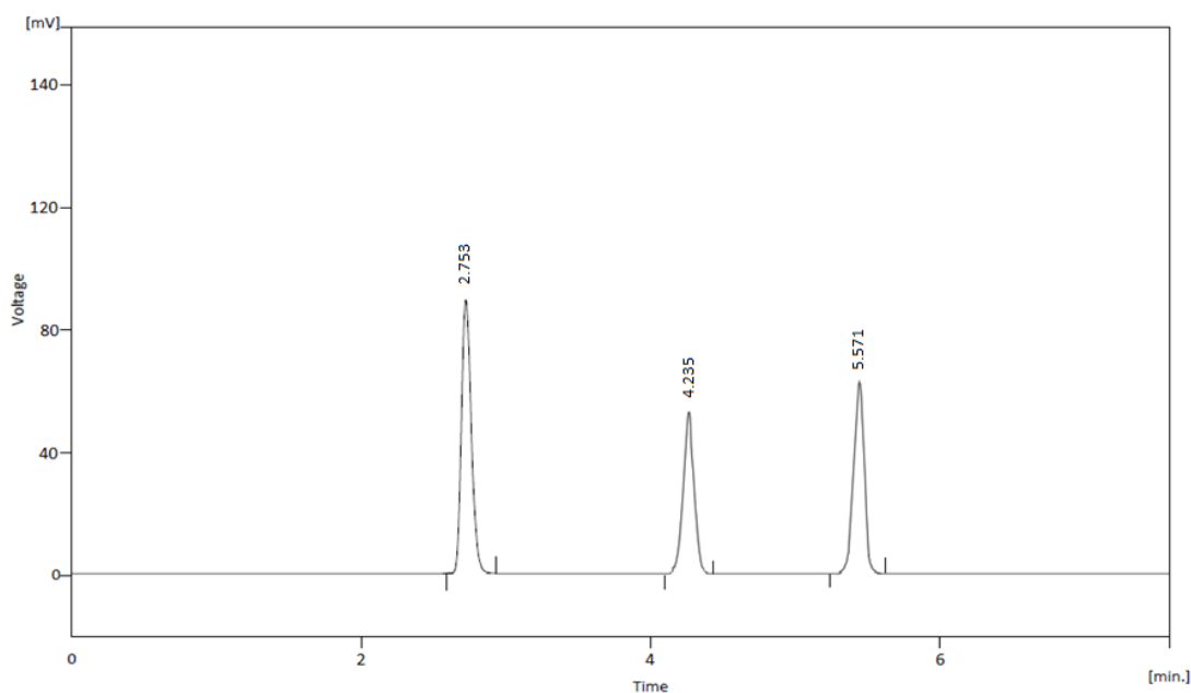
Figure 13.6: Chromatogram of Sample AMOX, CLAR & VONO
