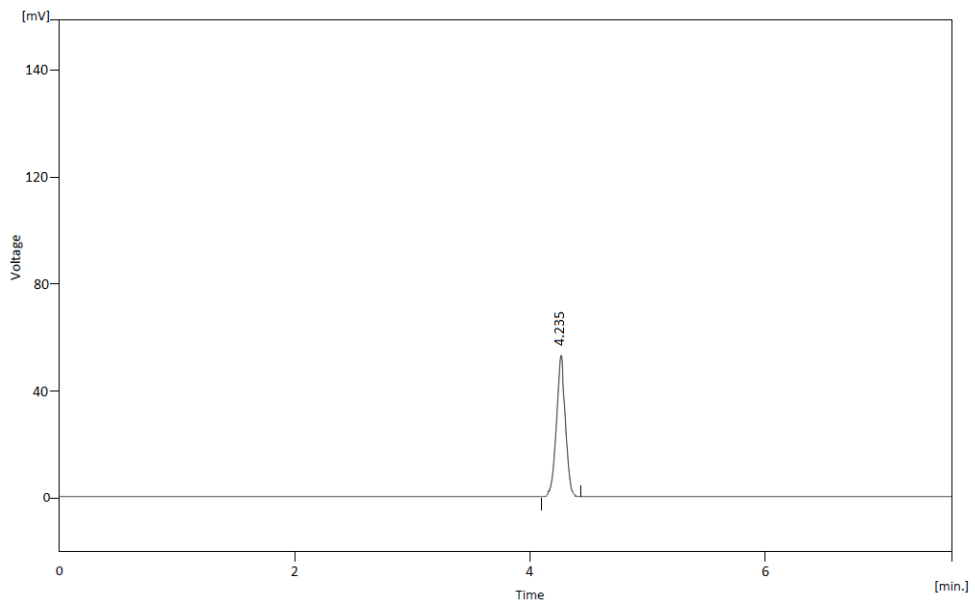
Figure 13.9: Chromatogram of CLAR
