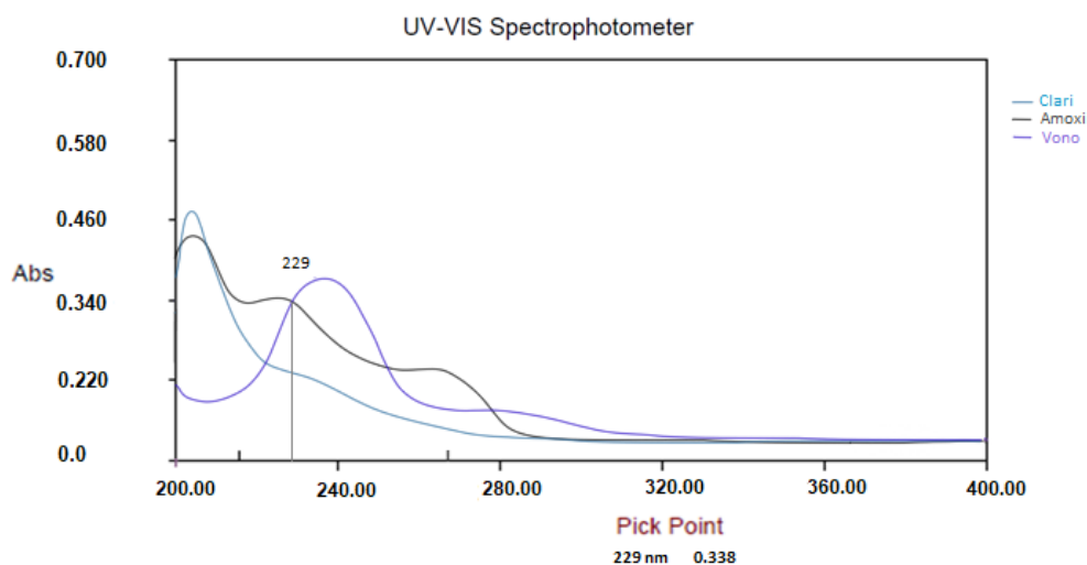
Figure 13.4: UV Spectra Overlay of AMOX, CLAR & VONO
