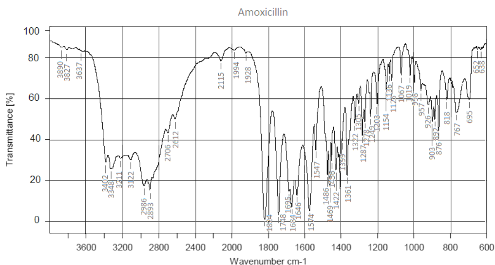
Figure 13.1: FTIR Spectra of Amoxicillin AMOX
