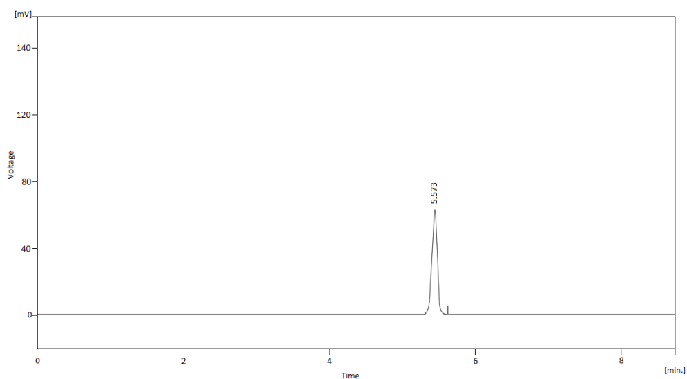
Figure 13.10: Chromatogram of VONO
