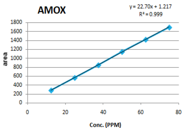
Figure 13.12: Calibration Curve for AMOX
