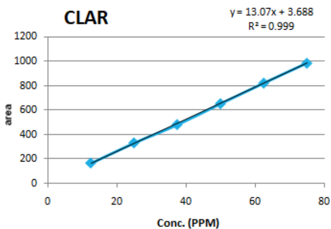
Figure 13.13: Calibration Curve for CLAR
