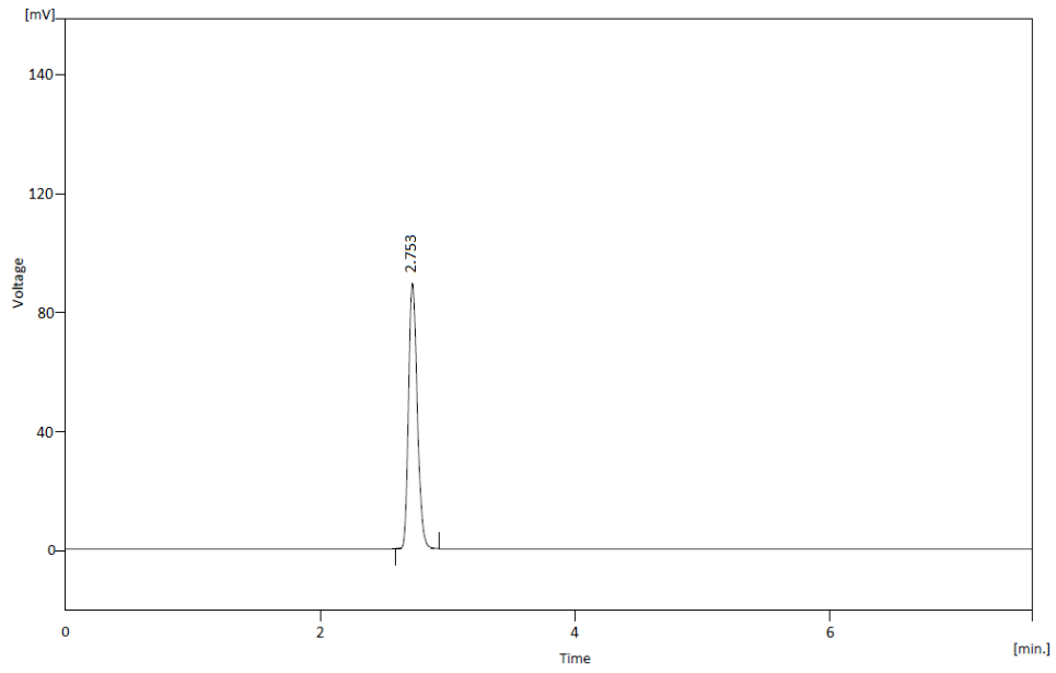
Figure 13.8: Chromatogram of AMOX
