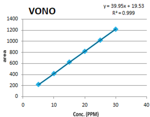
Figure 13.14: Calibration Curve for VONO
