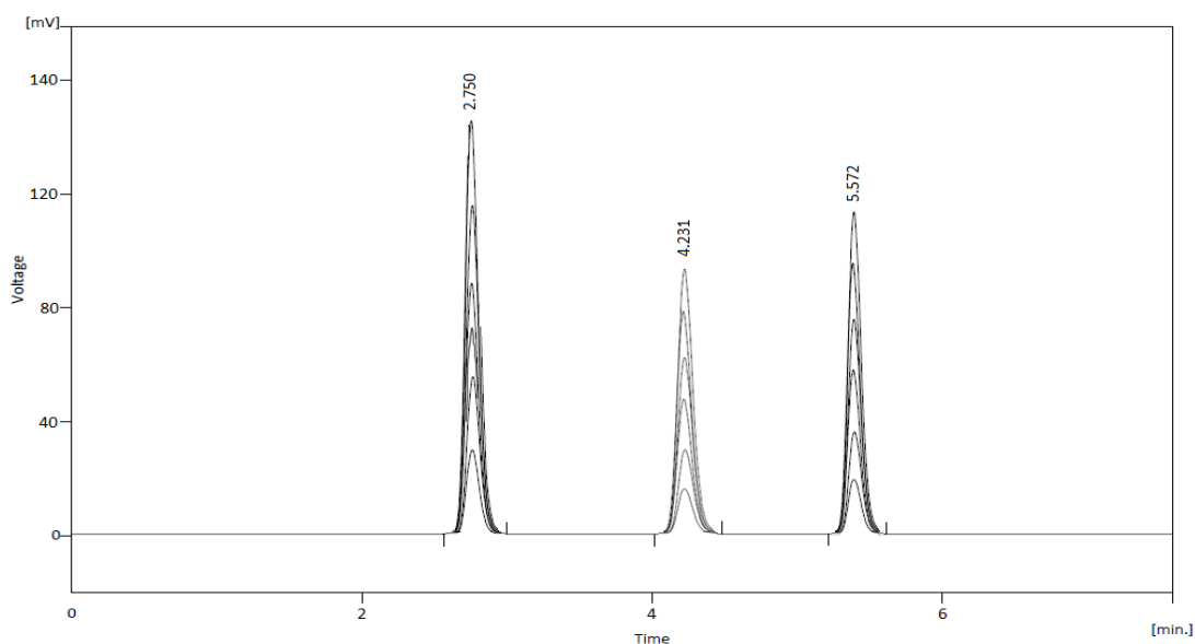
Figure 13.11: Overlain Chromatogram of Linearity for AMOX, CLAR &amp; VONO
