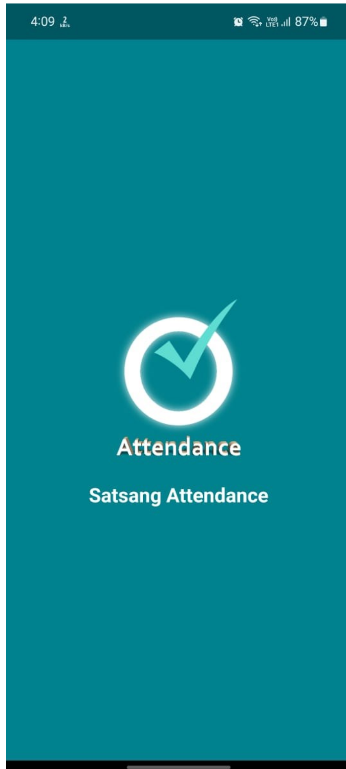
Fig.3.6. First interface
