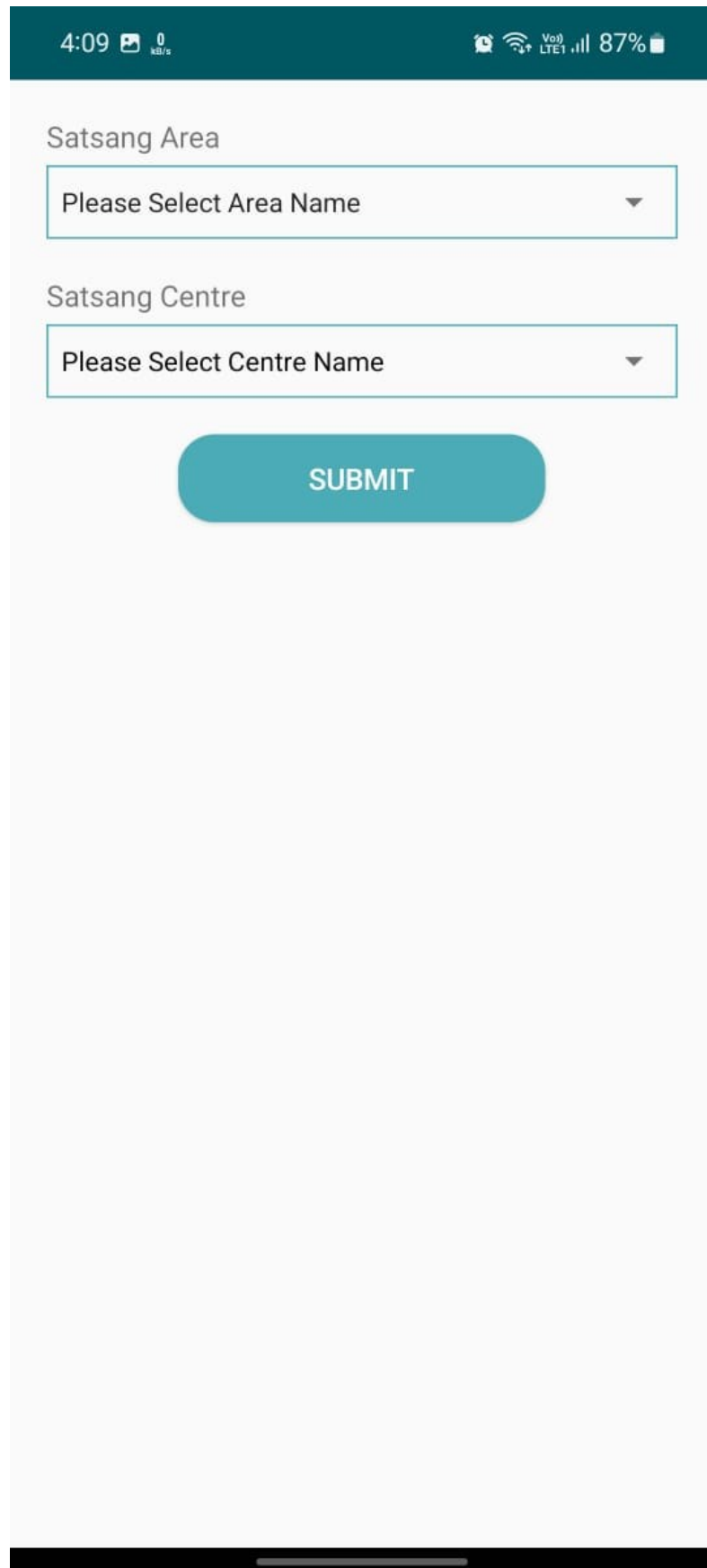
Fig.3.6.1 Home Page
