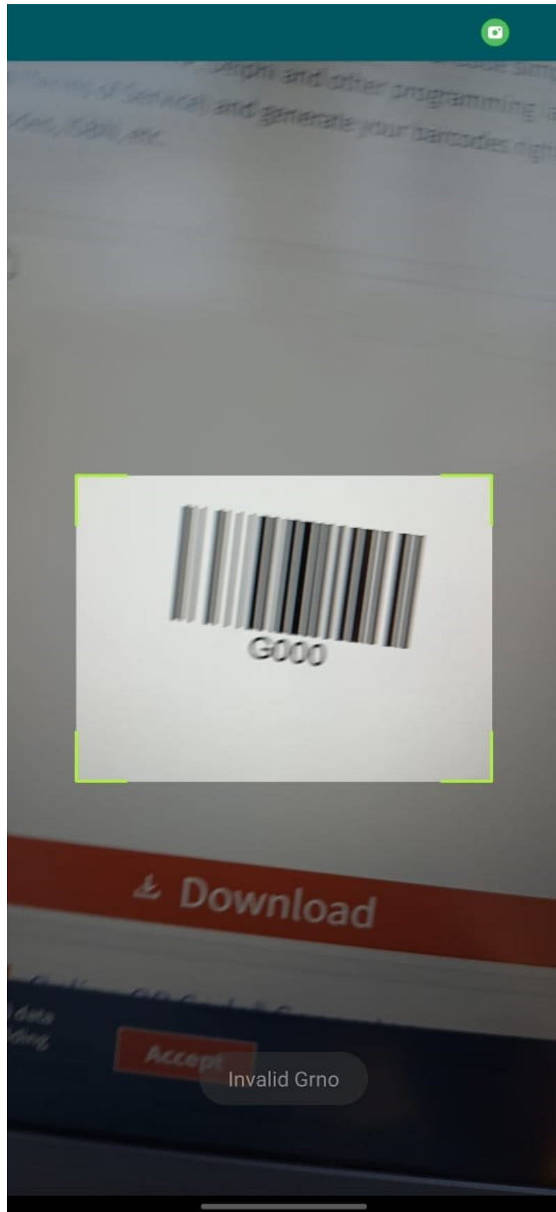
Fig.3.6.6 Scanner
