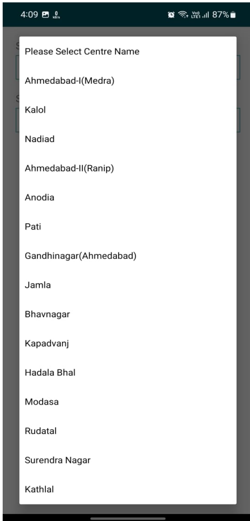
Fig.3.6.2 Choose area
