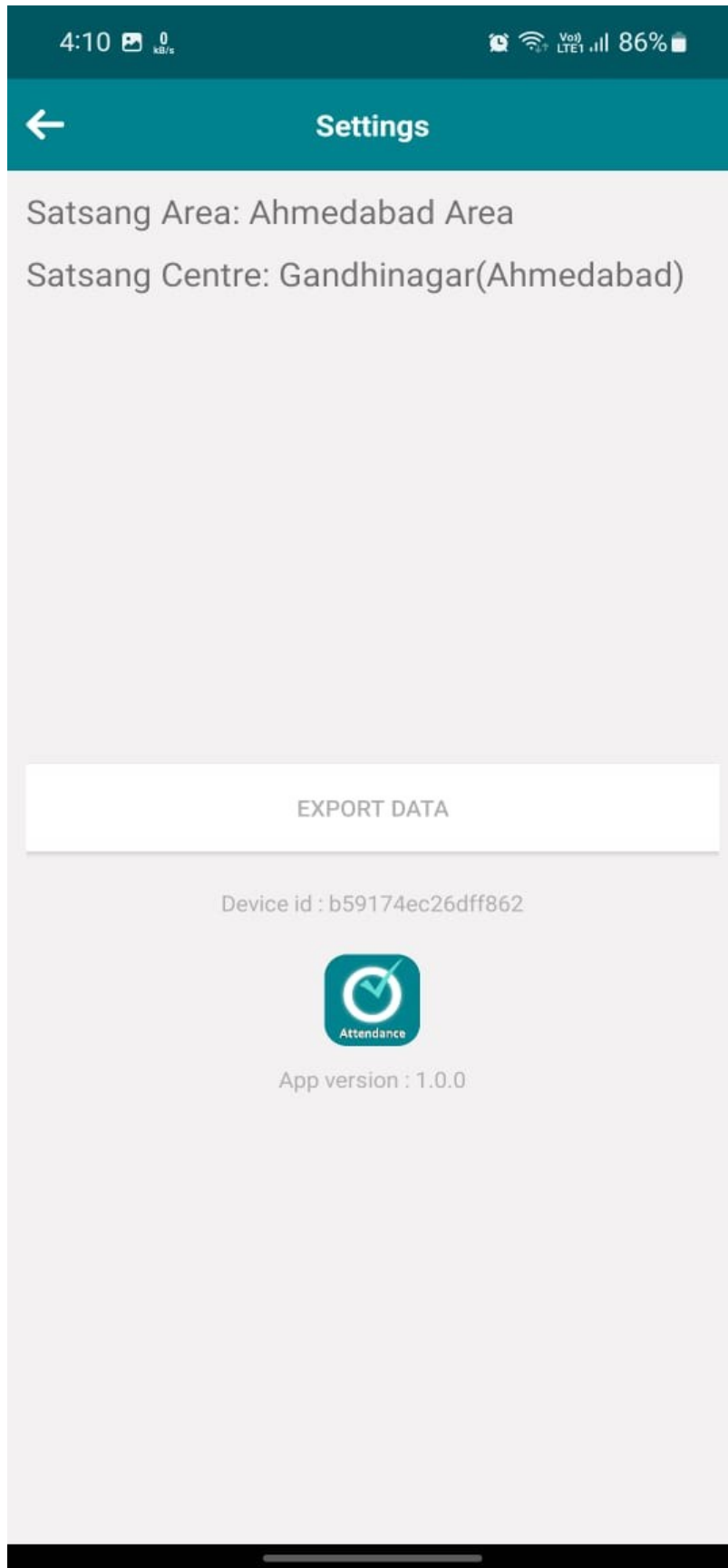
Fig.3.6.5 Export data
