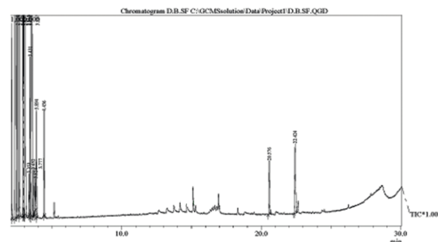
Figure 4. GC chromatogram of methyl ester fatty acid of C. dichotoma bark.
