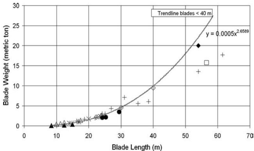
Fig. 2 Development in rotor blade weight versus length Symbols indicate different manufacturers and processing technologies
